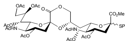
N -Acetyl-8- O -( N -acetyl-4',7',8',9',-tetra- O -acetyl-α-neuraminosyl)-2- S -phenyl-2-thio-neuraminic acid, 1',9-ester, 1-methyl-ester, 4,7-diacetate
