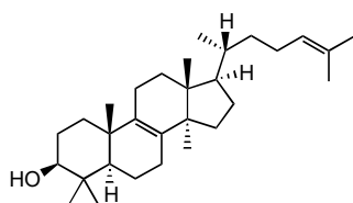
Lanosterol
