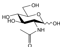
N + Acetyl-D-glucosamine
